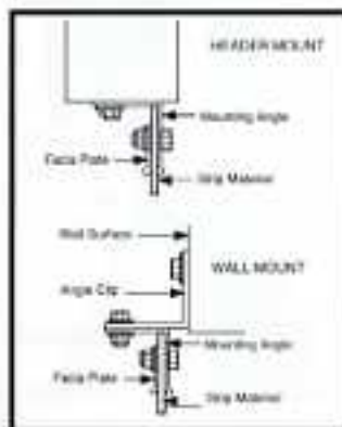
Galvanized Steel hardware Assembly
