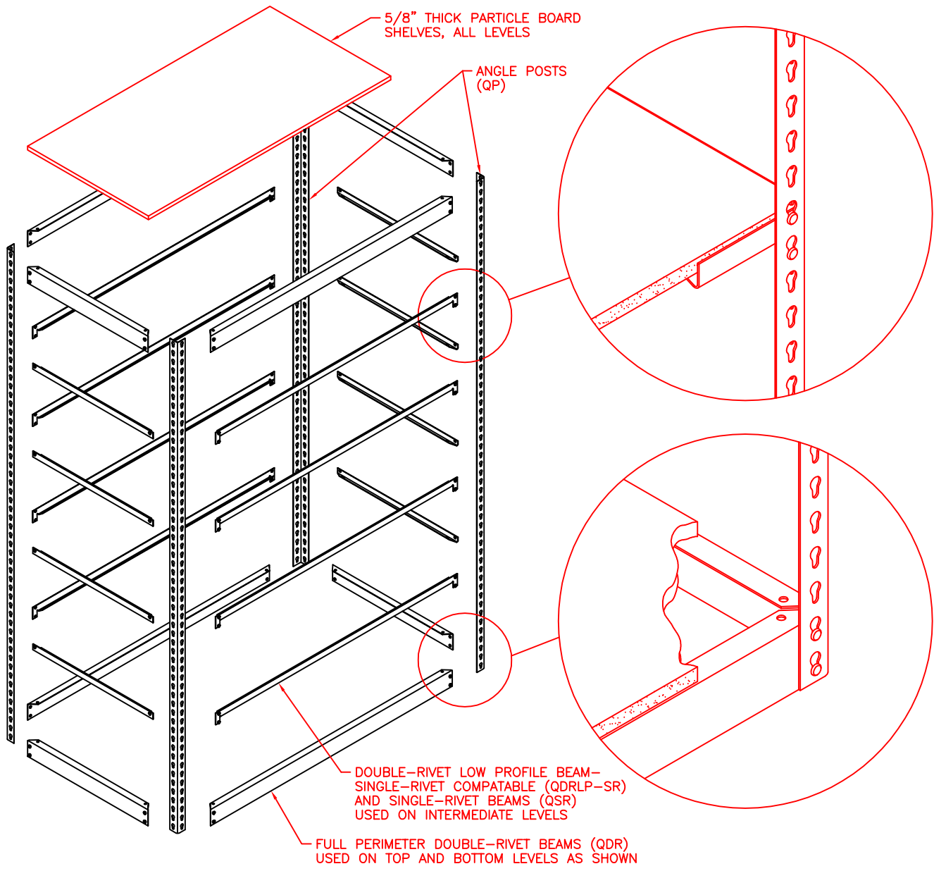
This is a Medium duty starter unit with 6 shelves
