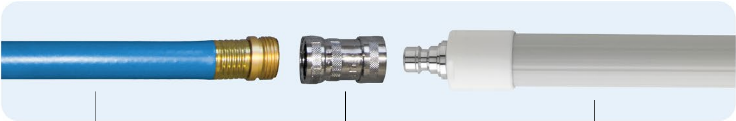
Standard US 3/4" Hose » 0703US - Automatic Shut-Off Coupling » 2973Qx - Waterfed telescopic handle
