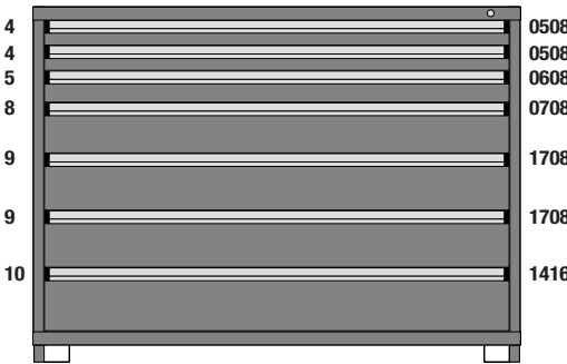
M1-602949FT-MD07AL • 7 Drawers • 238 Compartments
