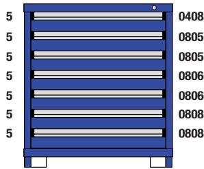
M1-302935FT-MD07AL • 7 Drawers • 152 Compartments
