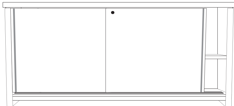
350 SERIES: WTL350 48"w x 28"d x 34"h WTL352 60"w x 28"d x 34"h WTL354 72"w x 28"d x 34"h Designed with 28" high doors to allow for cleaning under unit.
